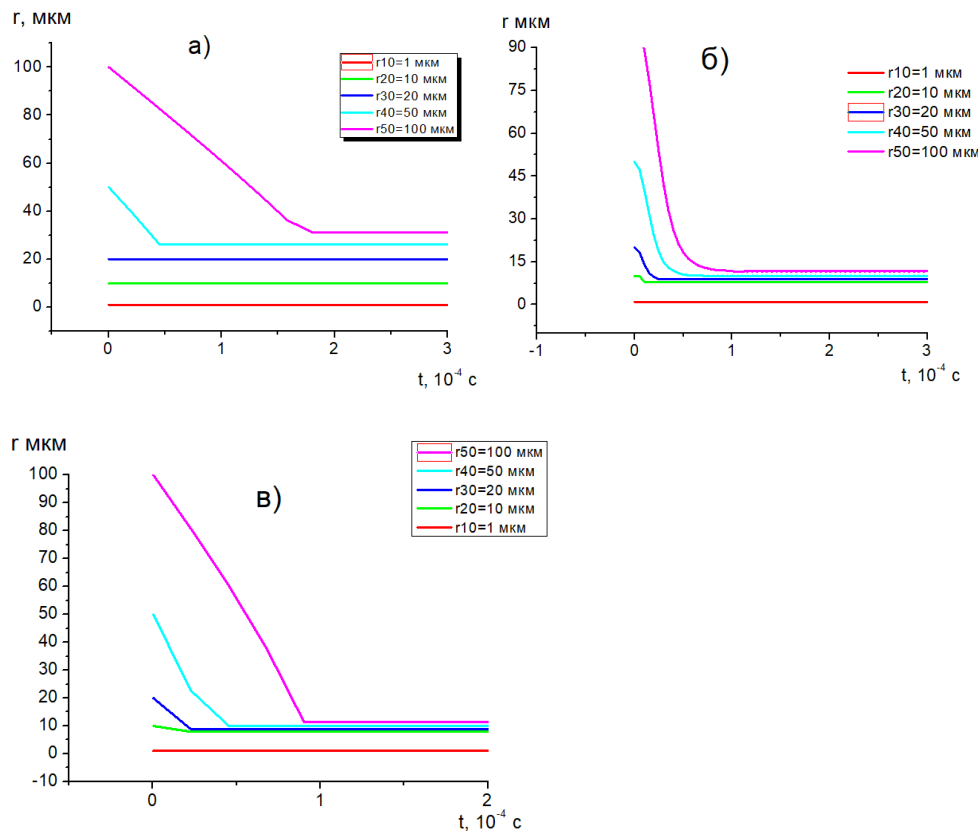
Figure 2 – Change of radii of five fractions from time at Mach numbers: a) M_1 = 0,15 ; б) M_2 = 0,25 ; в) M_3 = 0,40
