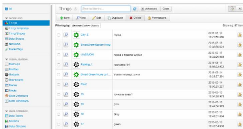
Figure 1. Thingworx interface
