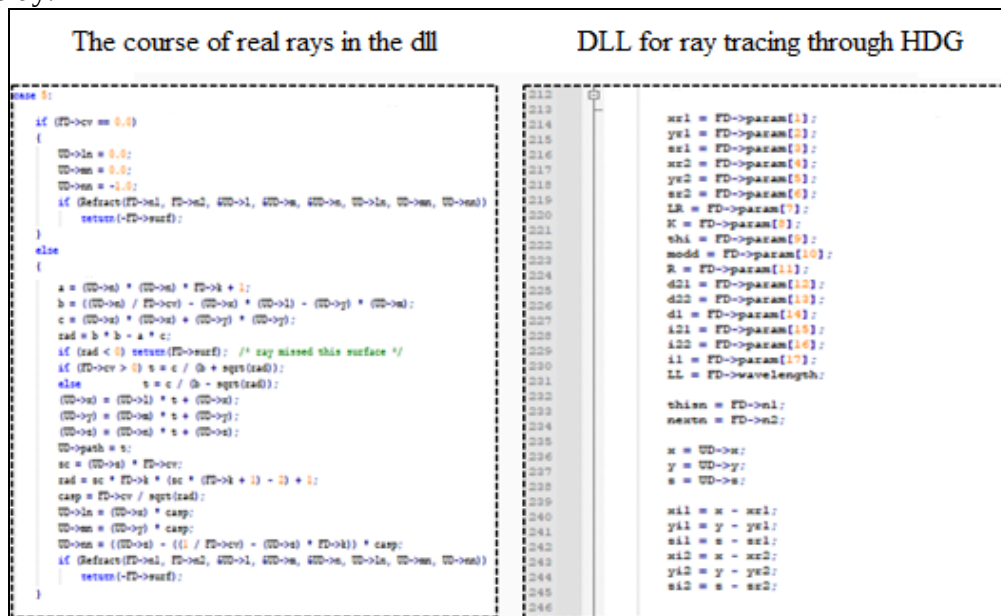
Fig.2. Software implementation of the code in the C programming language
