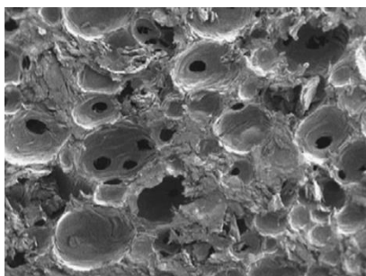
Figure 4. The structure of the CF containing graphite particles (5 wt.%)
