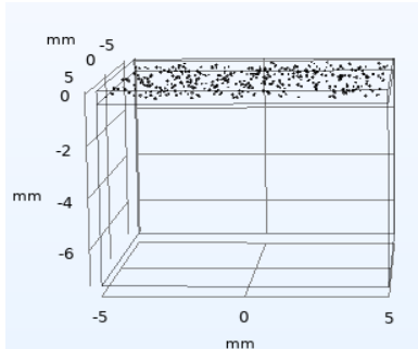
Figure 2. Geometry of a plate with randomized distribution of spheres and varying diameters
