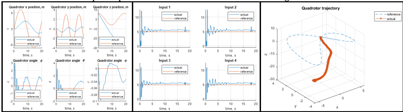
Figure 1. State and control changes and flight trajectory under the action of disturbances for 3D
