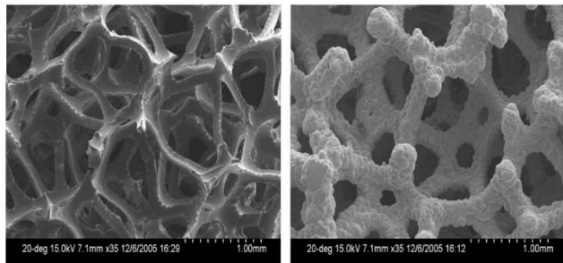
Figure 2. SEM image of CF:
