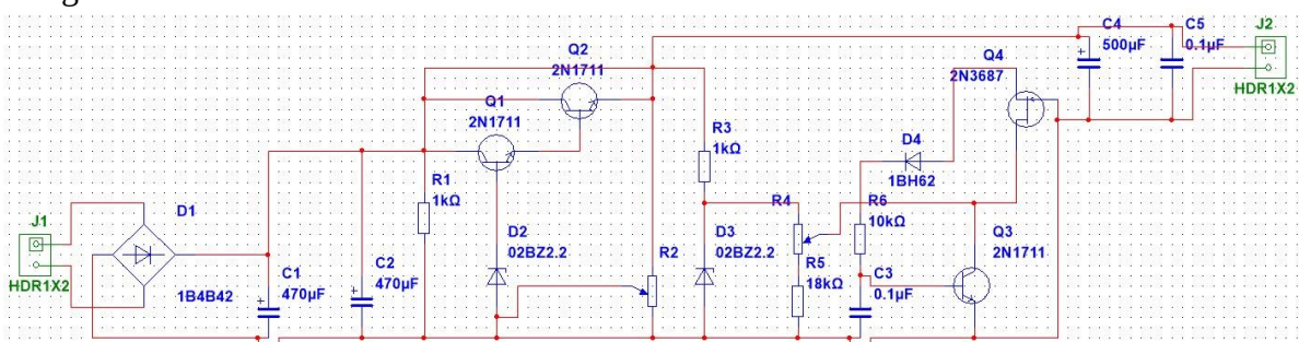
Figure 4 - Schematic diagram of the power supply unit for modeling in MultiSim
