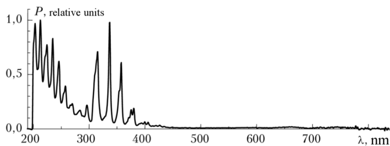
Fig. 1. Corona discharge emission spectrum
