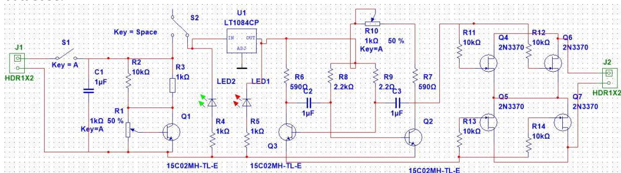
Figure 2 - Schematic diagram of the voltage converter block with indication elements for modeling in MultiSim
