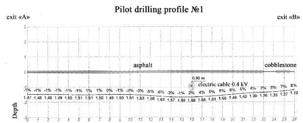
Fig. 8. Pilot drilling profile of cross-linked polyethylene insulated cable
