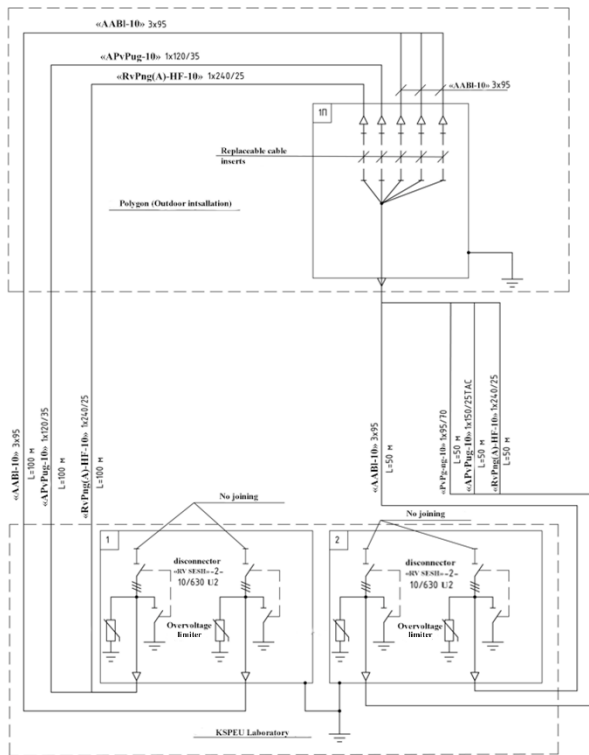
Fig. 6. Diagram of 10 kV cable lines polygon
