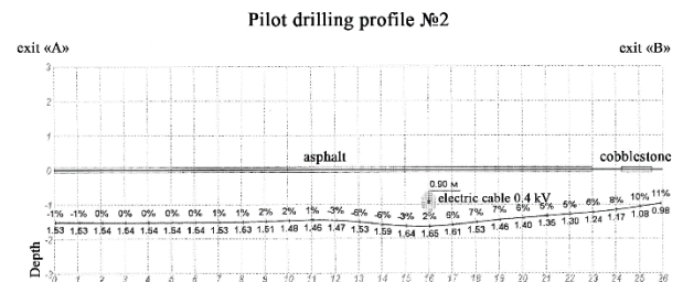
Fig. 9. Pilot drilling profile of paper-insulated cable
