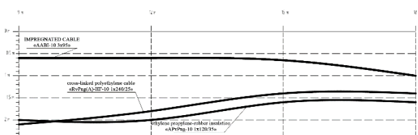
Fig. 12. The depth of the CL along the length in the second part in the section from 9 to 18 meters
