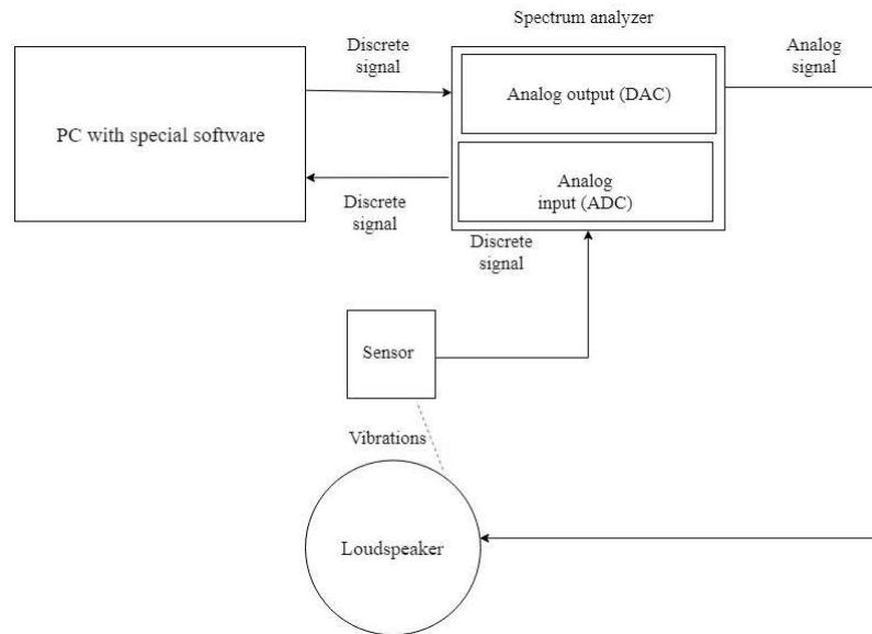
Figure 1. Scheme of the laboratory complex
