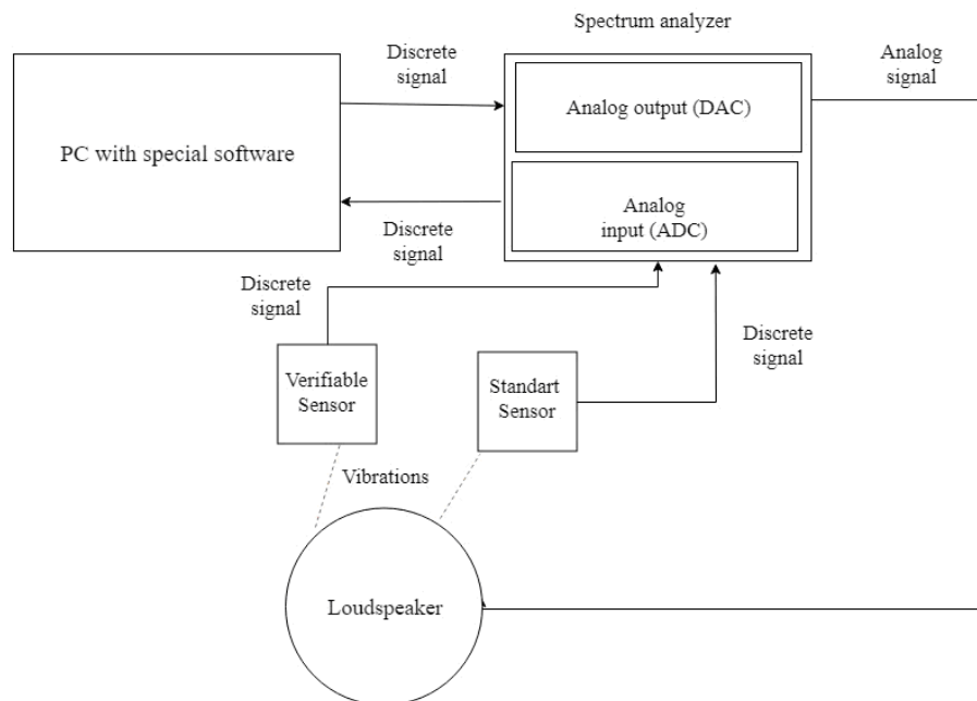
Figure 2. Installation diagram for sensor verification
